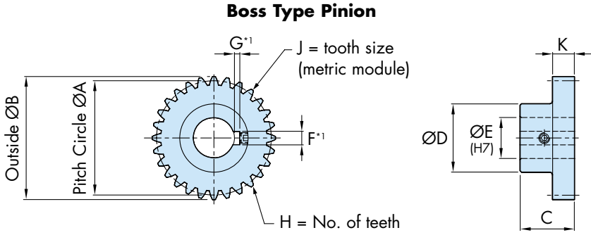
Boss Type Pinion
